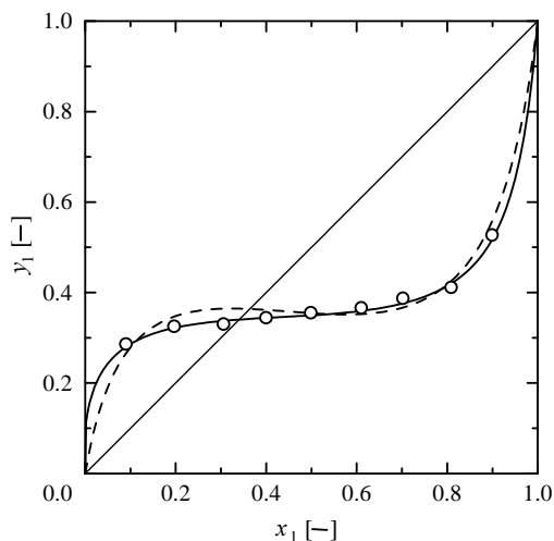
Fig.1 Correlation of vapor-liquid equilibria of ethanol(1) + hexane(2) binary system at 101.3kPa. Experimental 11) : (O);Correlations (—) with \alpha_{12}=0.827 , m_{12} = -0.0722 and n_{12} = -0.0189 ; (---) with \alpha_{12}= 1 , m_{12} = -0.0556 and n_{12} = -0.0478
