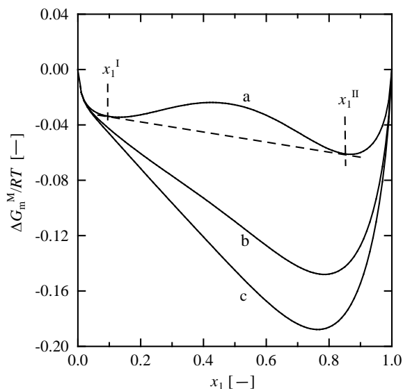
Fig. 2 Gibbs energies of mixing for heptane (1) + methanol (2) from GC-MW: (a) two liquid phase (25°C); (b) two liquid phase (50°C); (c) single liquid phase (60°C); x_1^{\text{I}} = 0.0990 and x_1^{\text{II}} = 0.8489
